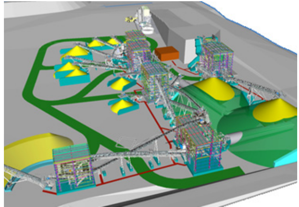
Plant design is based on flowsheet, layout, PFD, PID, functional description and more
